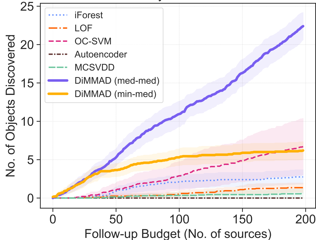
Anomaly: Mdwarf-flare
